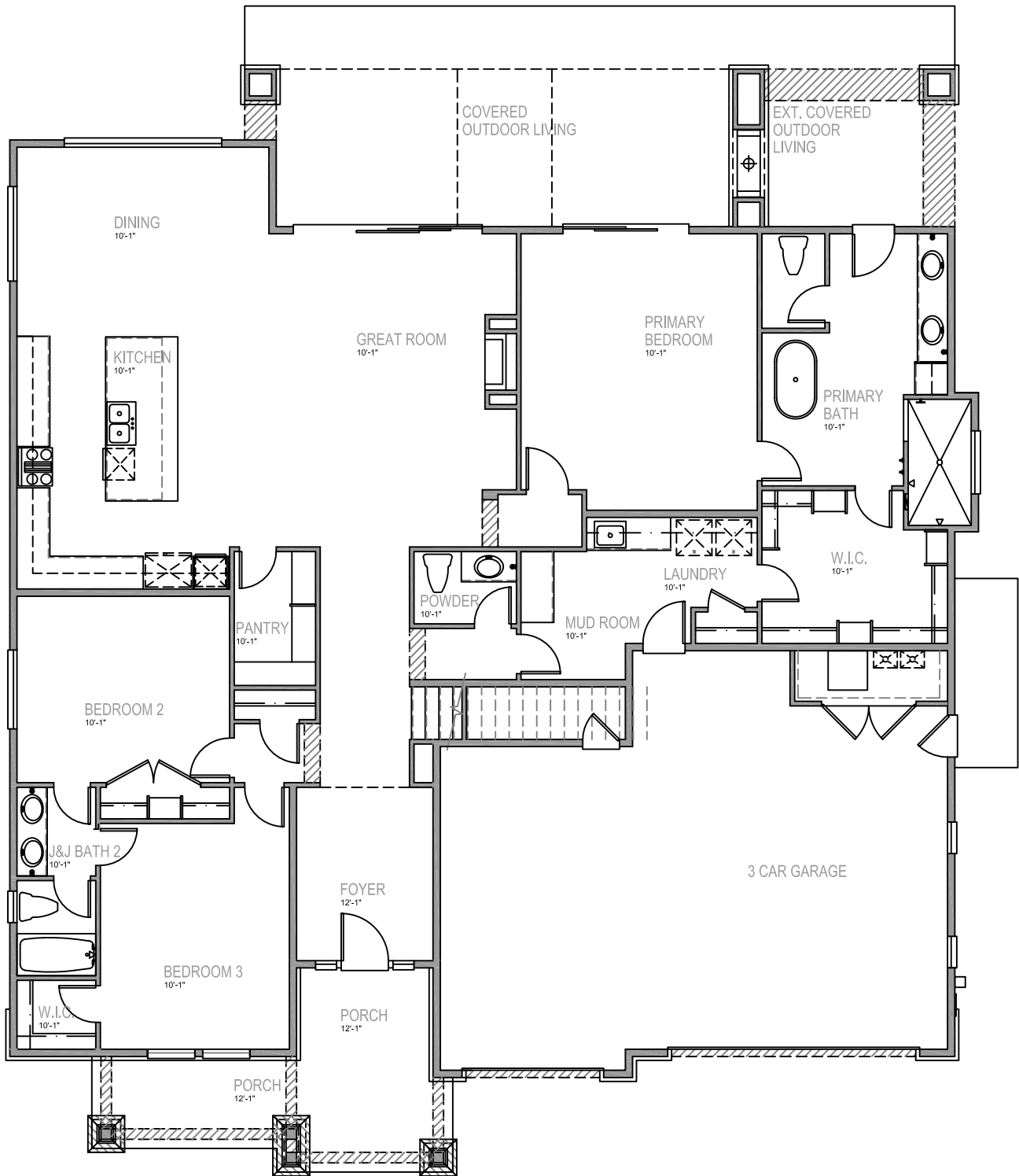
First Floor
